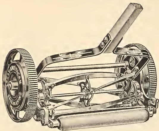
Great American Ball-Bearing Lawn Mower
